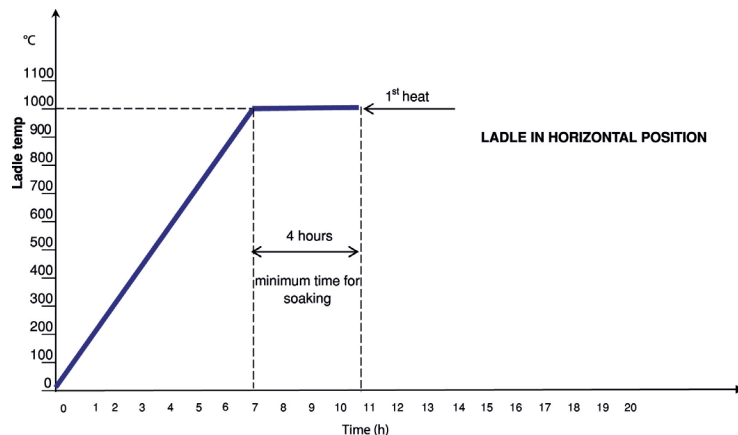
LADLE RE-HEATING CURVE
