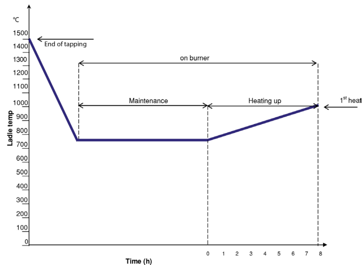
LADLE MAINTENANCE CURVE
